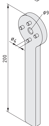
Stirnlochschlüssel 8 D25
