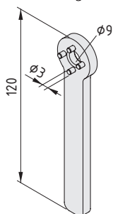
Stirnlochschlüssel 8 D14
